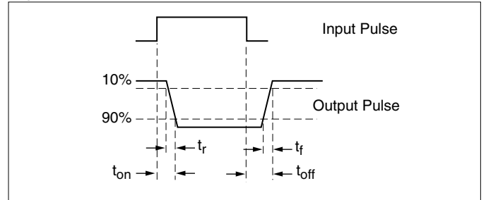
Figure 12. Test Circuit and Waveforms
