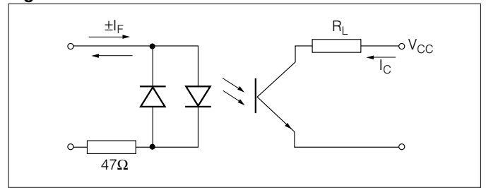
Figure 12. Test Circuit and Waveforms
